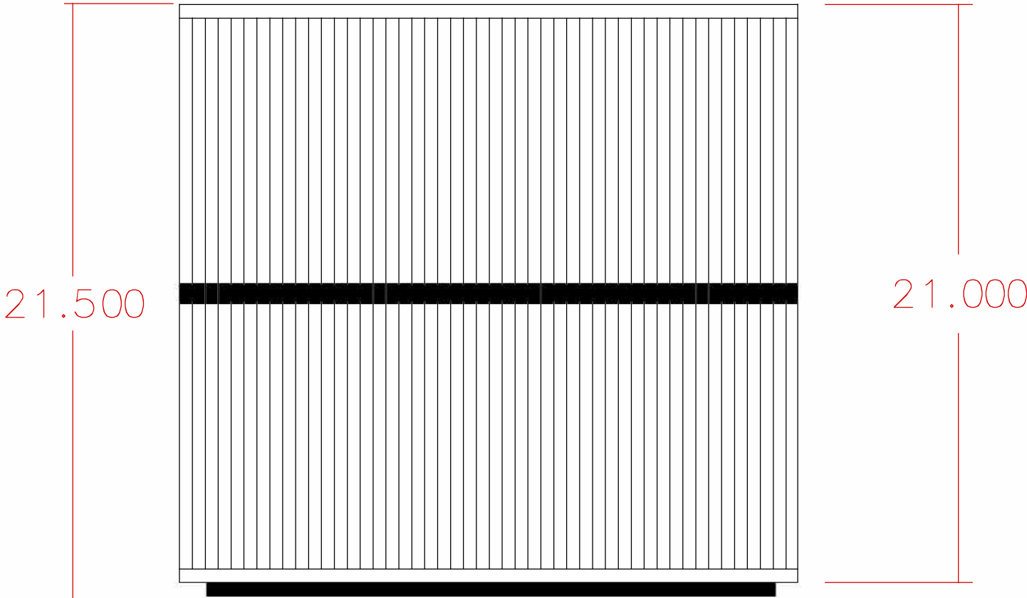
353 SQFT – 535 PLEATS FIRE RETARDANT MERV 15 NANOFIBER MEDIA
